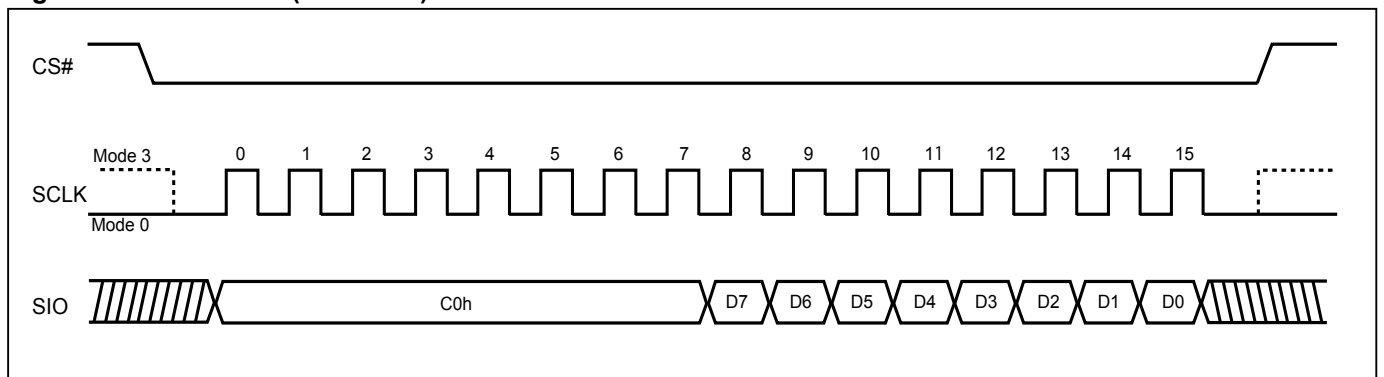
Figure 53. Burst Read (SPI Mode)
