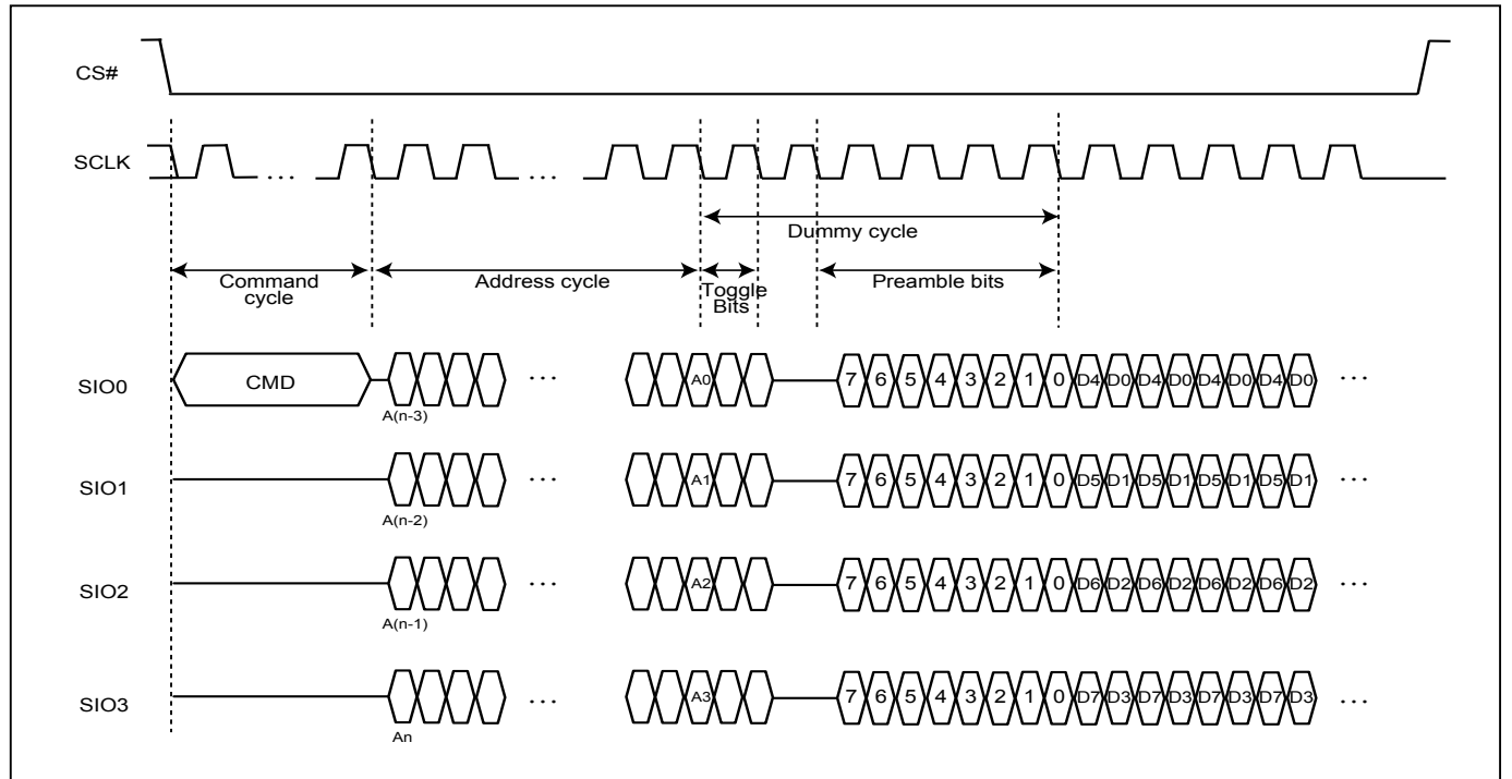
Figure 46. DTR4IO (6DC)
