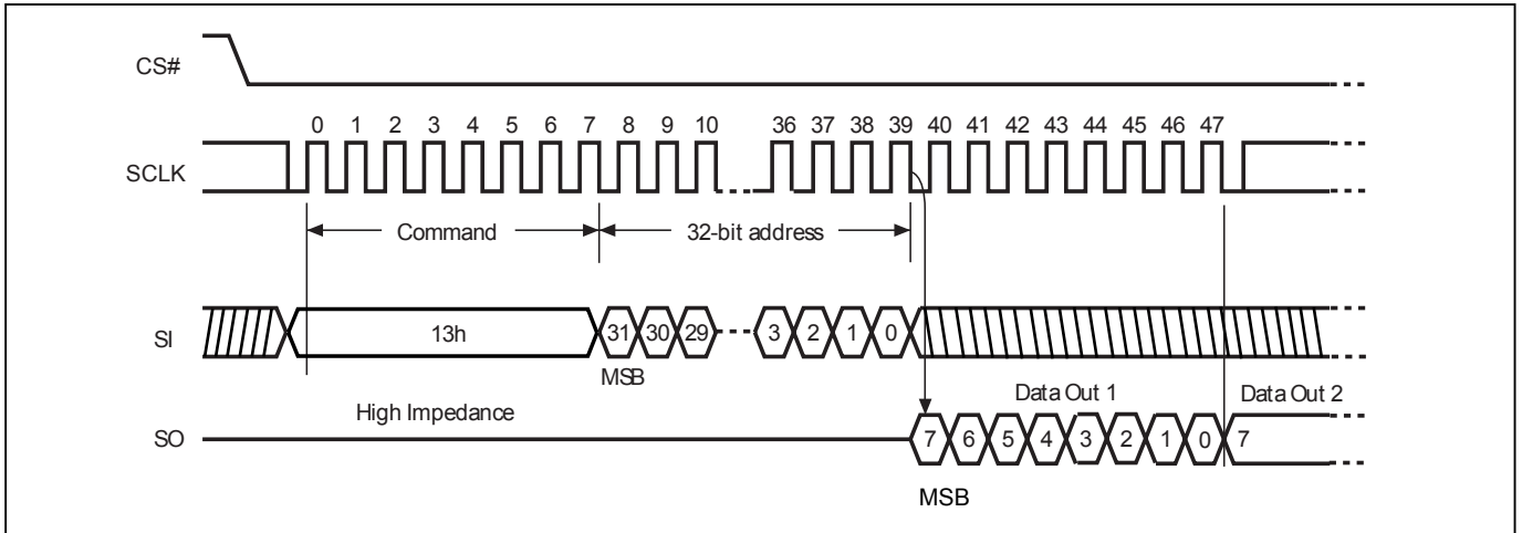
Figure 47. Read Data Bytes using 4-Byte Address Sequence (READ4B)
